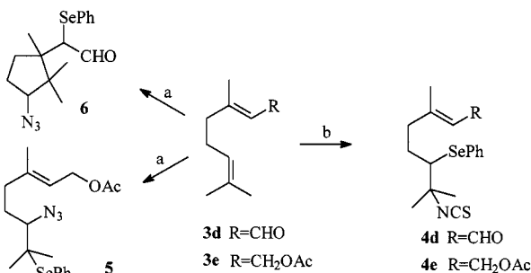
Scheme 5. Reagent and conditions: a. BAIB, (PhSe) 2 , NaN 3 , CH 2 Cl 2 , r.t., 12 h; b. BAIB, KSCN or TMSNCS, (PhSe) 2 , CH 3 CN or CH 2 Cl 2 , r.t., 2 h
