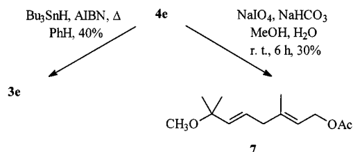
Scheme 6. Reductive and oxidative elimination of phenylselenium group from 4e
