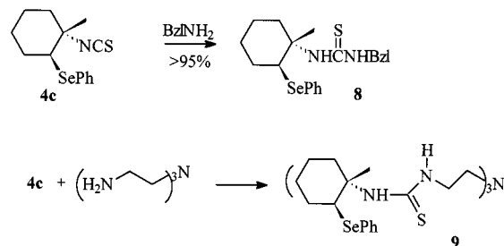
Scheme 7. Synthesis of N,N' -disubstituted thioureas
