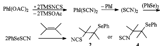
Scheme 4. Mechanism of phenylseleno-thiocyanation of olefins
